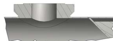
Studed olet
